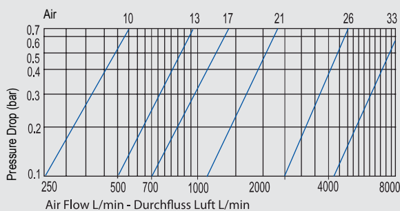
Flow Rate vs Pressure Drop Graph
