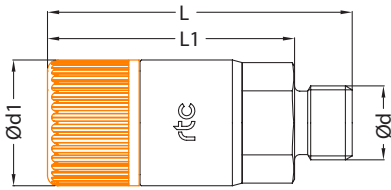
Socket / Kupplung
