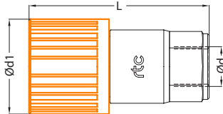
Socket / Kupplung
