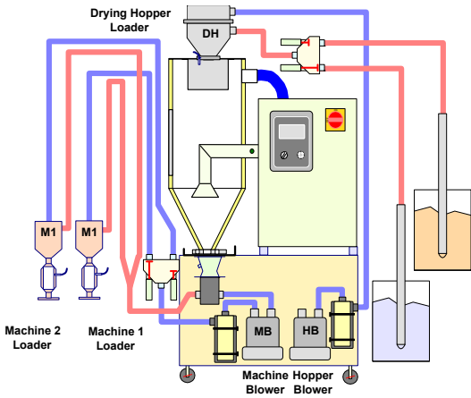
Convey to Drying Hopper With Proportioning Valve & Two Machines, Configuration "DP"
