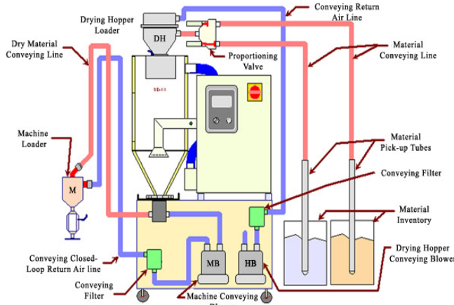
Convey to Drying Hopper With Proportioning Valve & Two Machines, Configuration "CP"
