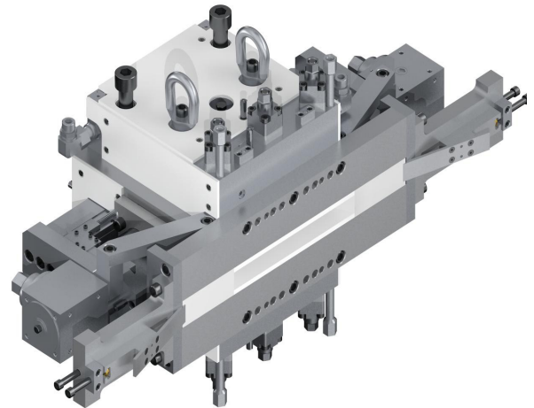
330mm XPS Foam Board Die with Forming Box
